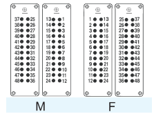
接插针排序 Contacts arrangement view from termination side
