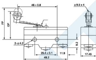
CBLM-25(30)
